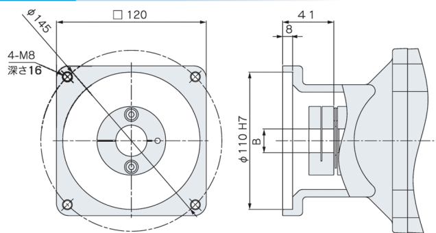
図8 0.75kW T2, T4
