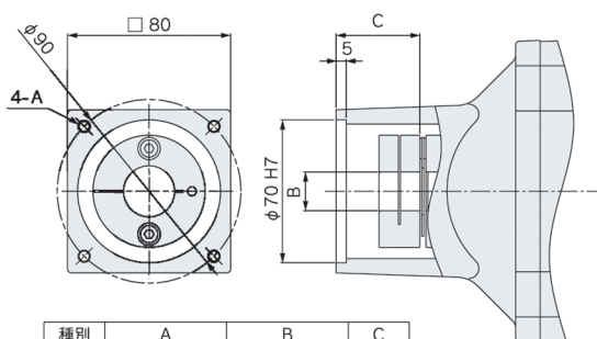
図7 0.75kW T1, T3, T5
